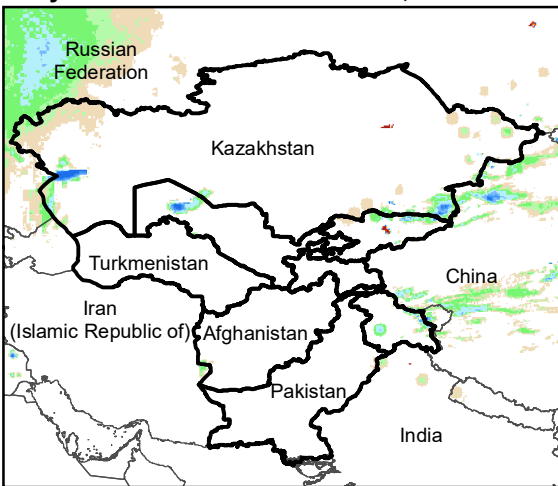
Daily Rainfall estimate for 20 Jan., 2012
