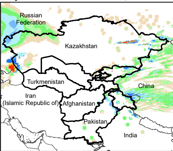
Daily Rainfall estimate for 19 Jan., 2012
