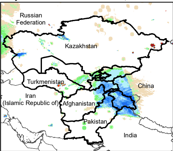
Daily Rainfall estimate for 18 Jan., 2012
