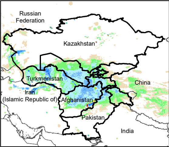
Daily Rainfall estimate for 6 Feb., 2012
