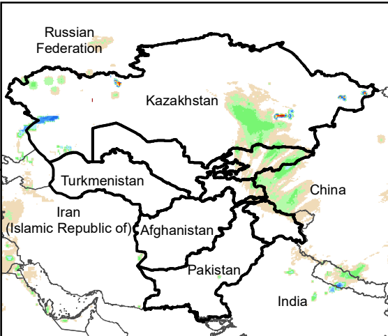
Daily Rainfall estimate for 7 Feb., 2012
