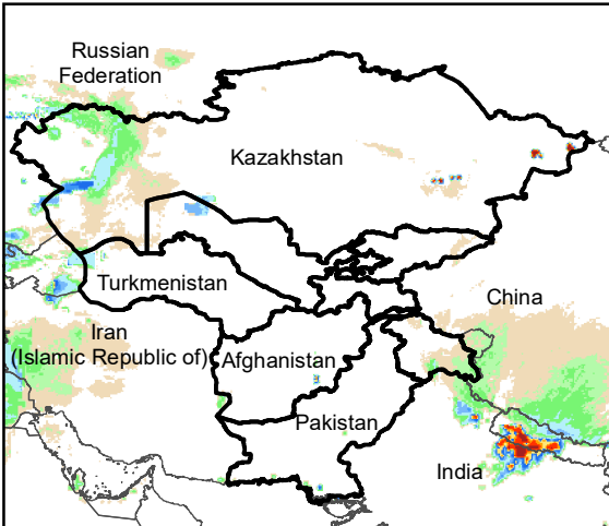
Daily Rainfall estimate for 8 Feb., 2012
