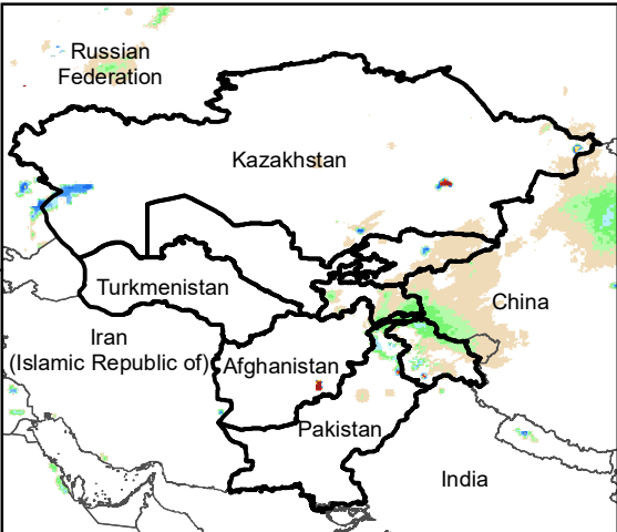
Daily Rainfall estimate for 22 Feb., 2012
