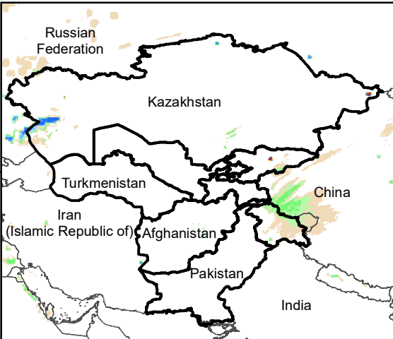
Daily Rainfall estimate for 23 Feb., 2012
