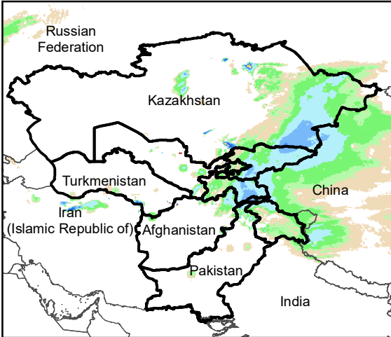
Daily Rainfall estimate for 24 Feb., 2012
