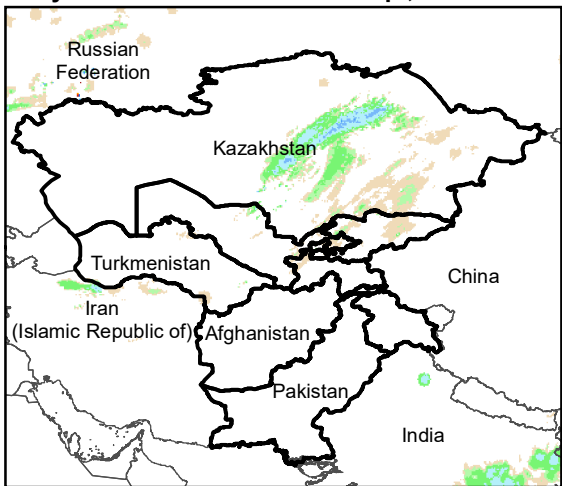
Daily Rainfall estimate for 2 Oct., 2012
