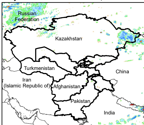
Daily Rainfall estimate for 1 Oct., 2012
