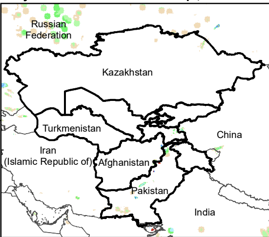
Daily Rainfall estimate for 30 Sep., 2012
