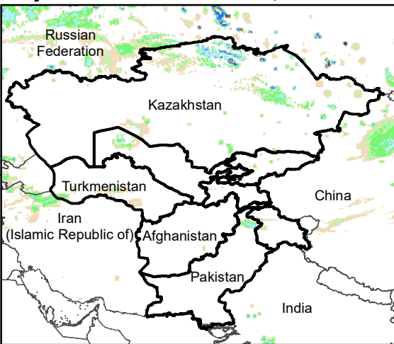
Daily Rainfall estimate for 10 Oct., 2012
