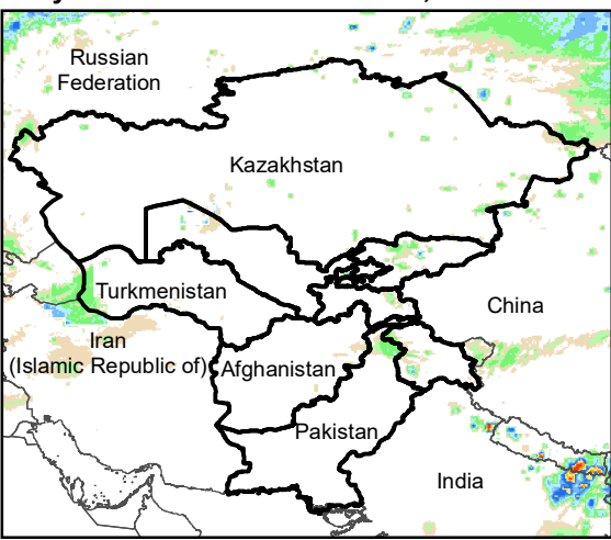
Daily Rainfall estimate for 9 Oct., 2012
