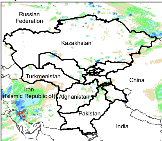
Daily Rainfall estimate for 27 Nov., 2012
