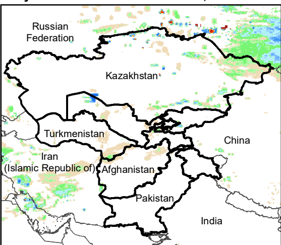
Daily Rainfall estimate for 25 Nov., 2012
