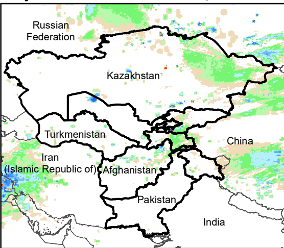
Daily Rainfall estimate for 26 Nov., 2012
