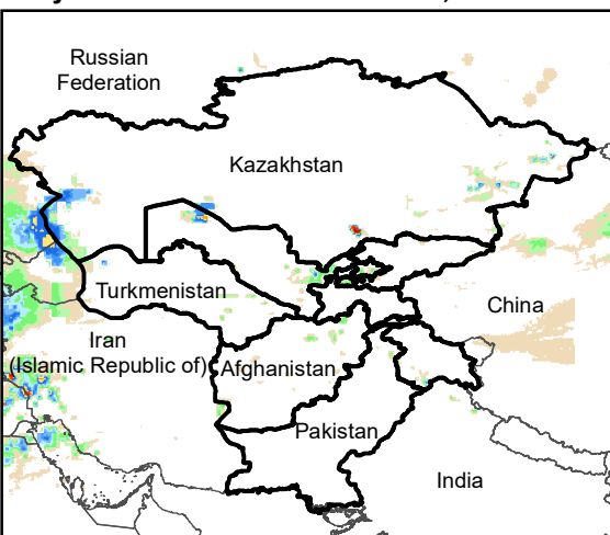
Daily Rainfall estimate for 20 Dec., 2012
