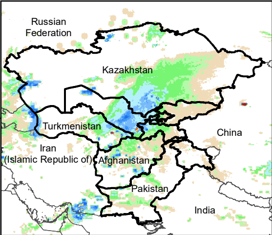
Daily Rainfall estimate for 5 Feb., 2013
