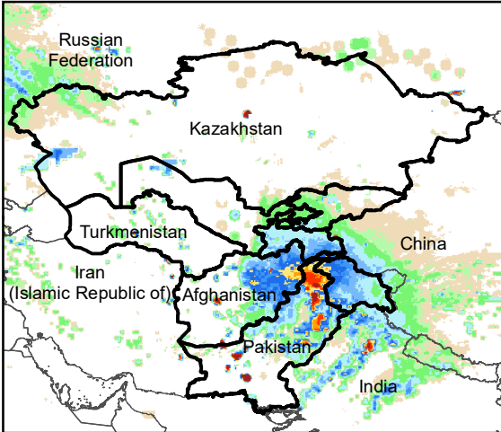
Daily Rainfall estimate for 7 Feb., 2013
