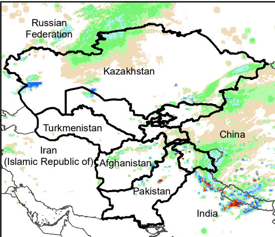
Daily Rainfall estimate for 6 Feb., 2013
