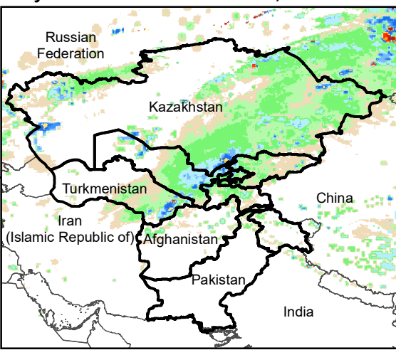
Daily Rainfall estimate for 3 Mar., 2013
