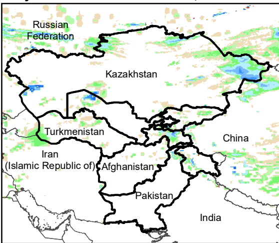
Daily Rainfall estimate for 4 Mar., 2013
