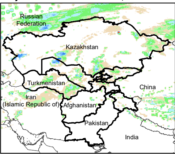
Daily Rainfall estimate for 2 Mar., 2013
