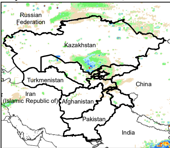
Daily Rainfall estimate for 29 Oct., 2013
