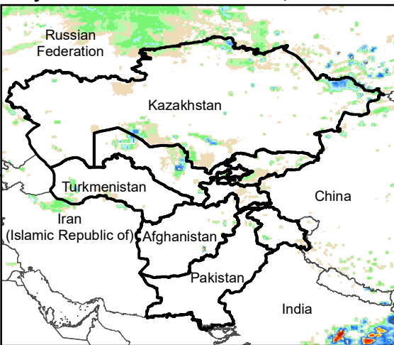
Daily Rainfall estimate for 28 Oct., 2013
