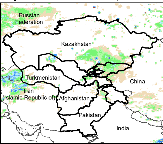
Daily Rainfall estimate for 27 Oct., 2013
