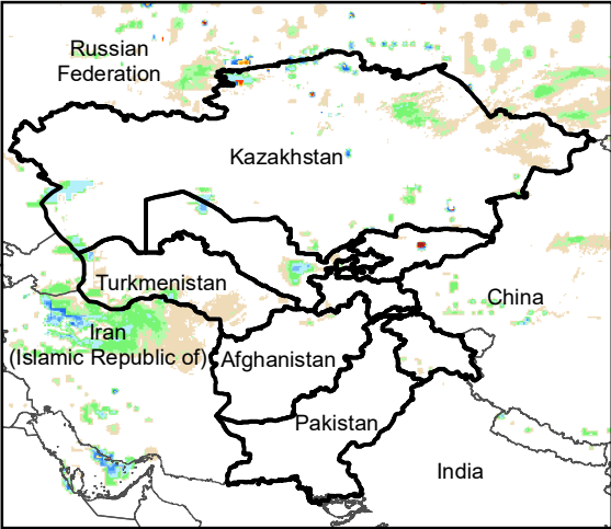
Daily Rainfall estimate for 5 Jan., 2014
