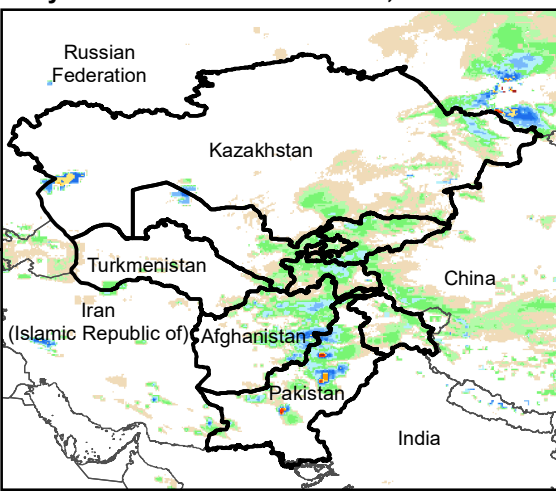
Daily Rainfall estimate for 7 Mar., 2014
