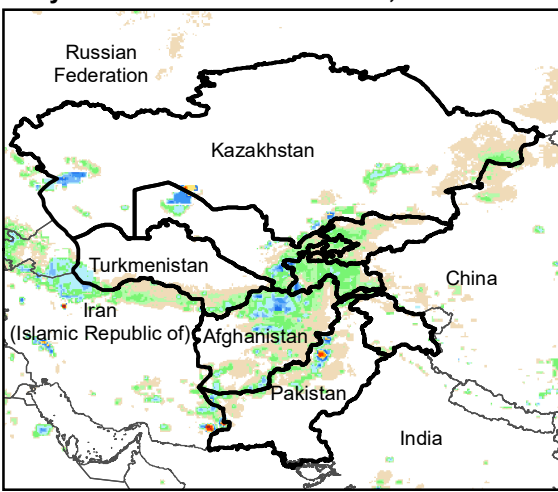
Daily Rainfall estimate for 8 Mar., 2014
