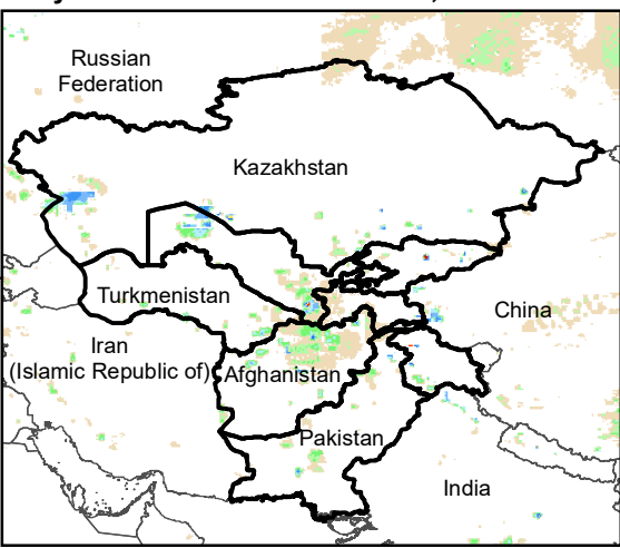
Daily Rainfall estimate for 6 Mar., 2014
