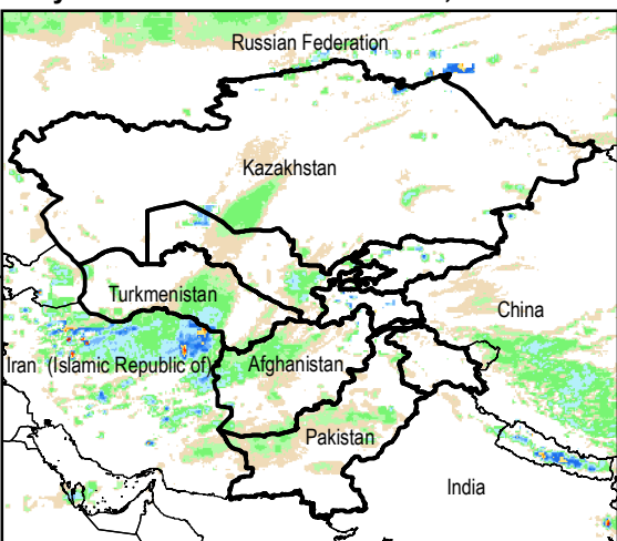
Daily Rainfall estimate for 22 Mar., 2014
