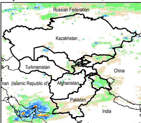
Daily Rainfall estimate for 26 Mar., 2014
