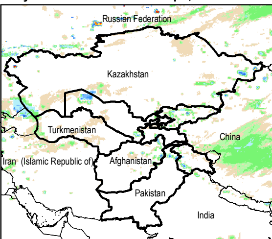
Daily Rainfall estimate for 9 Apr., 2014
