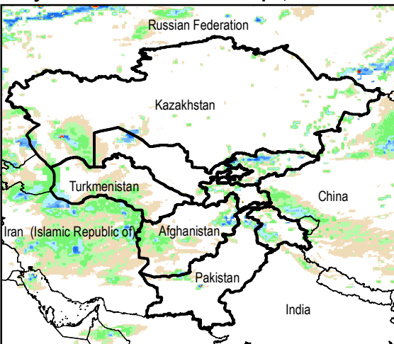
Daily Rainfall estimate for 26 Apr., 2014
