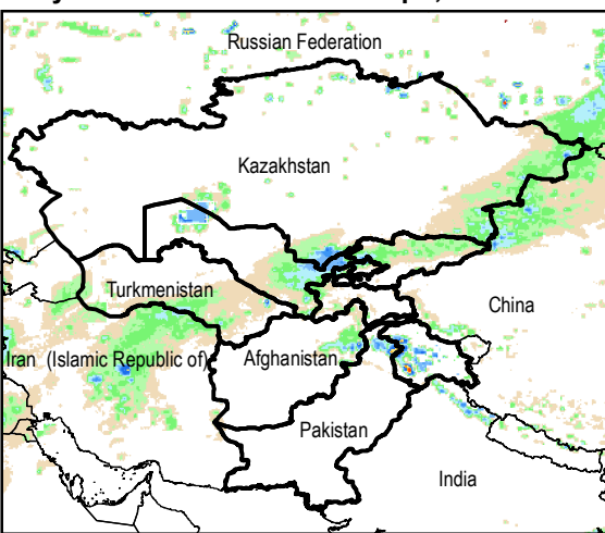
Daily Rainfall estimate for 28 Apr., 2014
