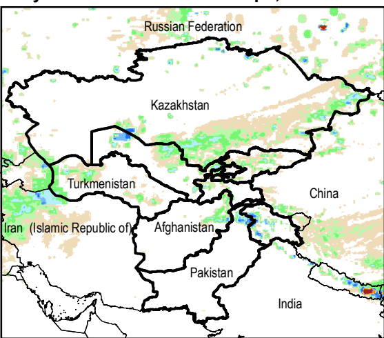
Daily Rainfall estimate for 27 Apr., 2014
