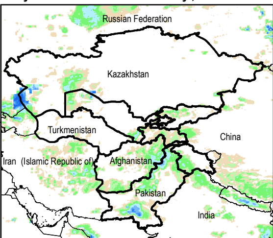
Daily Rainfall estimate for 4 May., 2014
