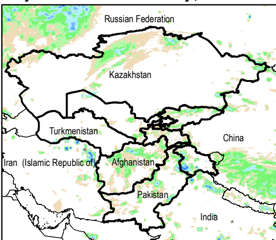
Daily Rainfall estimate for 6 May., 2014
