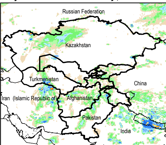
Daily Rainfall estimate for 5 May., 2014
