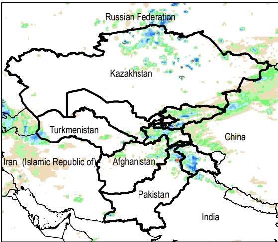
Daily Rainfall estimate for 20 May., 2014
