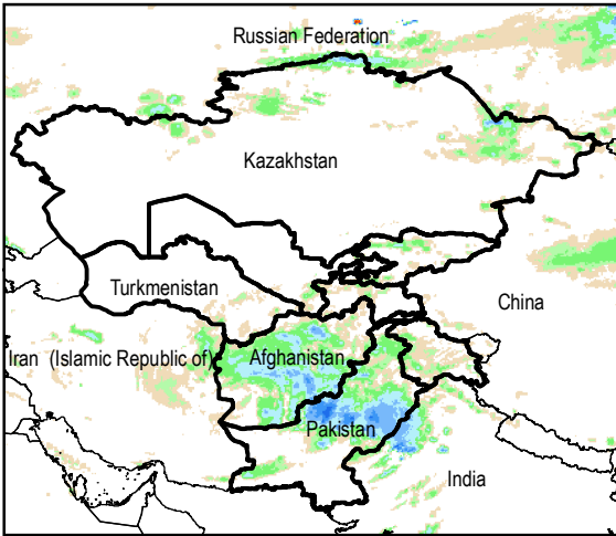
Daily Rainfall estimate for 20 May., 2014
