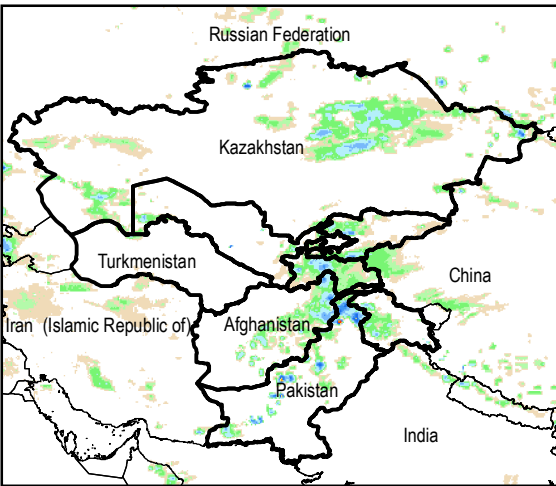
Daily Rainfall estimate for 19 May., 2014
