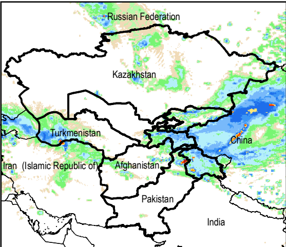
Daily Rainfall estimate for 22 May., 2014
