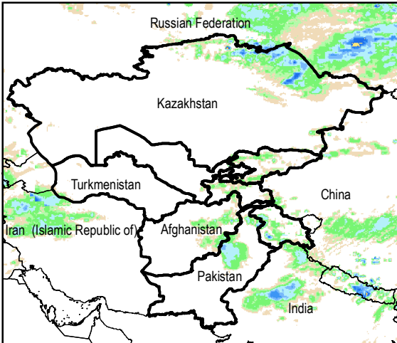
Daily Rainfall estimate for 24 May., 2014
