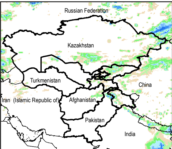
Daily Rainfall estimate for 8 Jun., 2014
