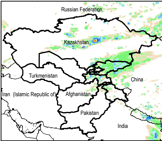
Daily Rainfall estimate for 10 Jun., 2014
