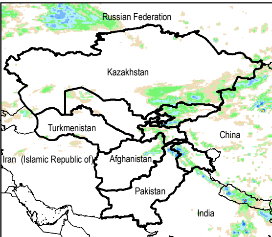
Daily Rainfall estimate for 9 Jun., 2014
