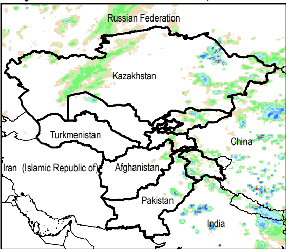
Daily Rainfall estimate for 27 Jun., 2014
