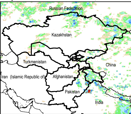
Daily Rainfall estimate for 28 Jun., 2014
