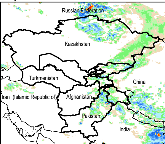
Daily Rainfall estimate for 5 Jul., 2014
