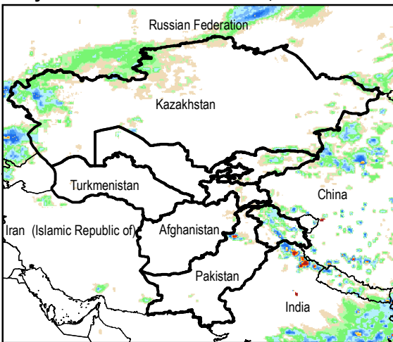
Daily Rainfall estimate for 11 Jul., 2014
