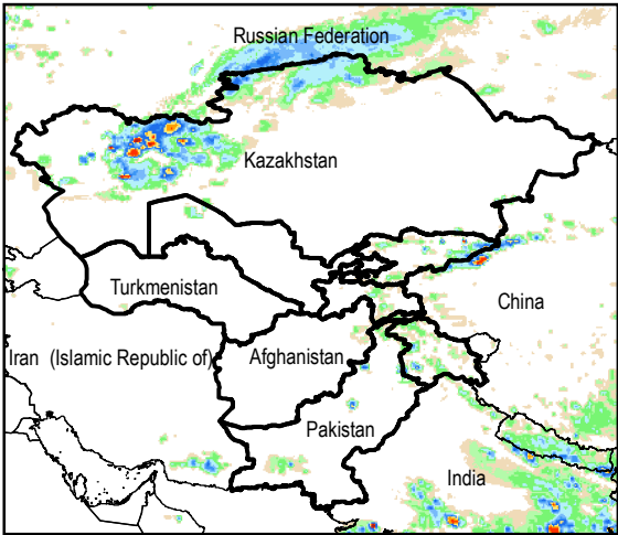
Daily Rainfall estimate for 13 Jul., 2014
