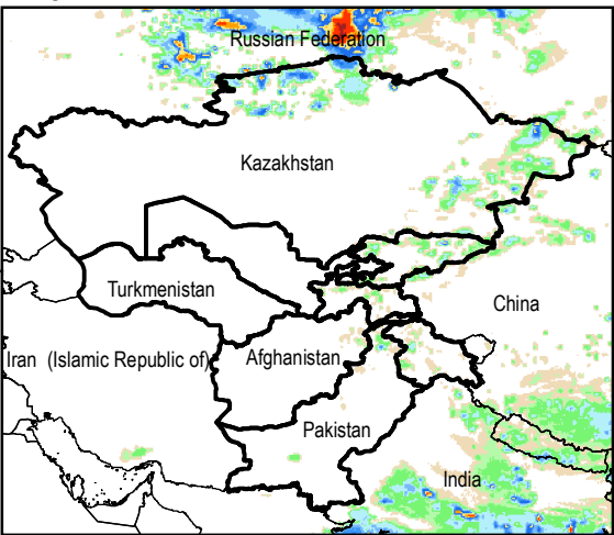
Daily Rainfall estimate for 12 Jul., 2014
