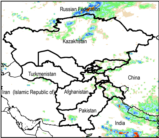
Daily Rainfall estimate for 14 Jul., 2014
