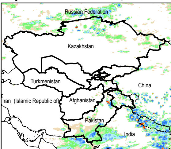
Daily Rainfall estimate for 25 Jul., 2014
