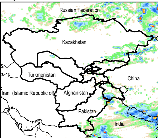
Daily Rainfall estimate for 26 Jul., 2014
