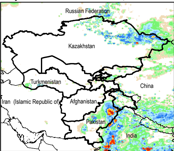
Daily Rainfall estimate for 1 Aug., 2014
