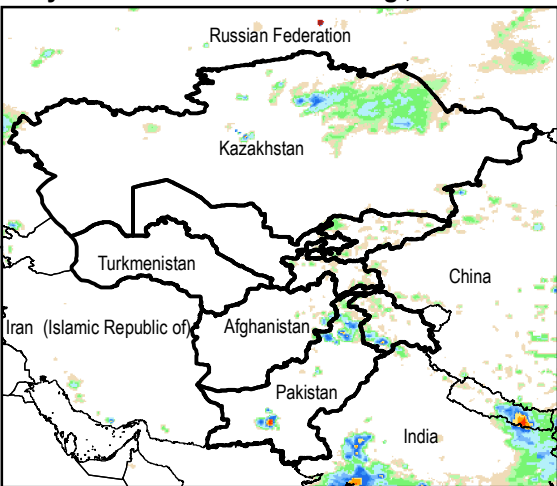
Daily Rainfall estimate for 28 Aug., 2014
