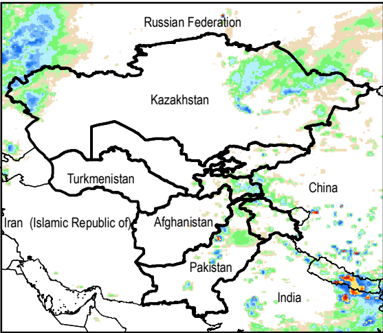
Daily Rainfall estimate for 29 Aug., 2014
