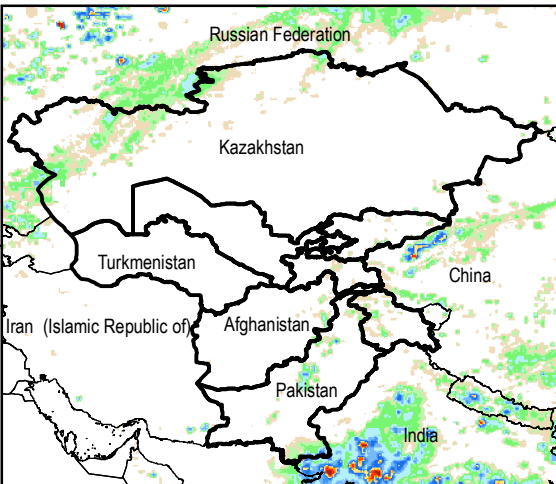
Daily Rainfall estimate for 30 Aug., 2014
