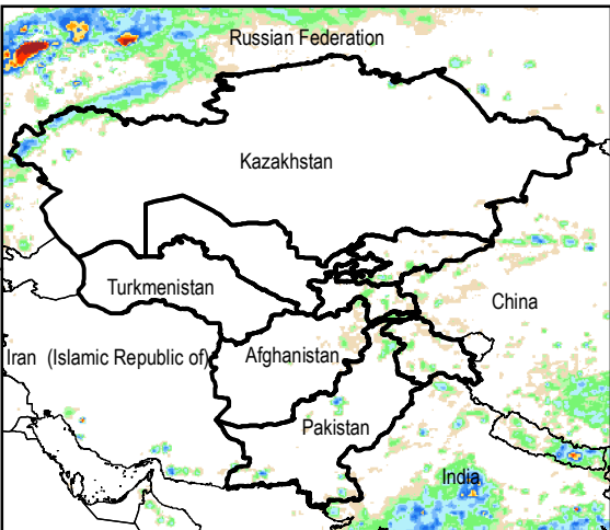
Daily Rainfall estimate for 29 Aug., 2014
