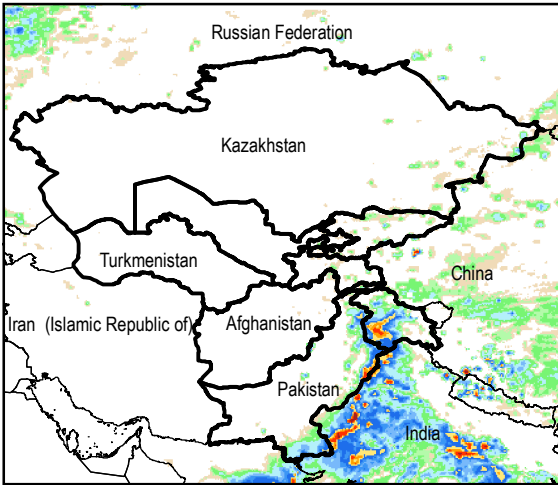
Daily Rainfall estimate for 6 Sep., 2014
