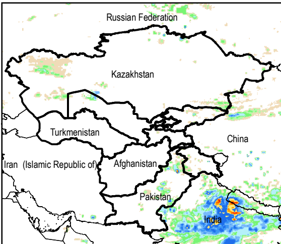
Daily Rainfall estimate for 11 Sep., 2014
