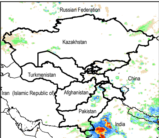
Daily Rainfall estimate for 9 Sep., 2014
