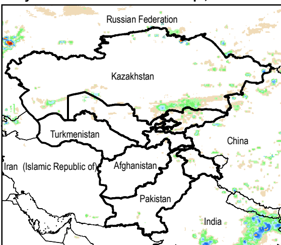
Daily Rainfall estimate for 15 Sep., 2014
