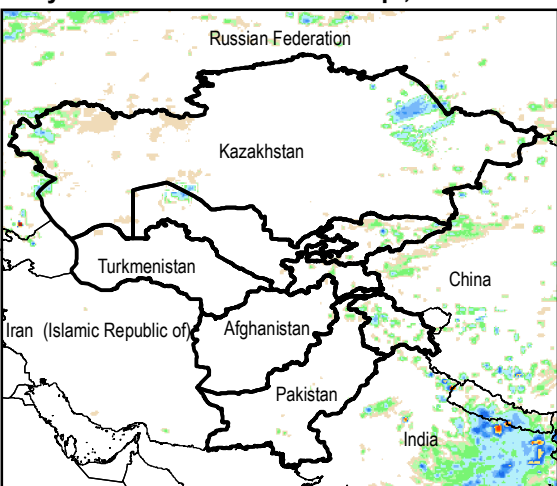
Daily Rainfall estimate for 13 Sep., 2014
