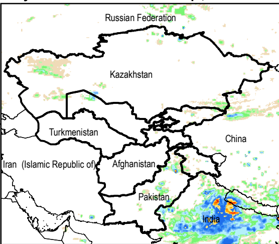
Daily Rainfall estimate for 14 Sep., 2014
