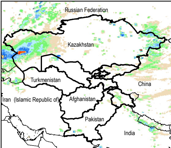
Daily Rainfall estimate for 29 Sep., 2014
