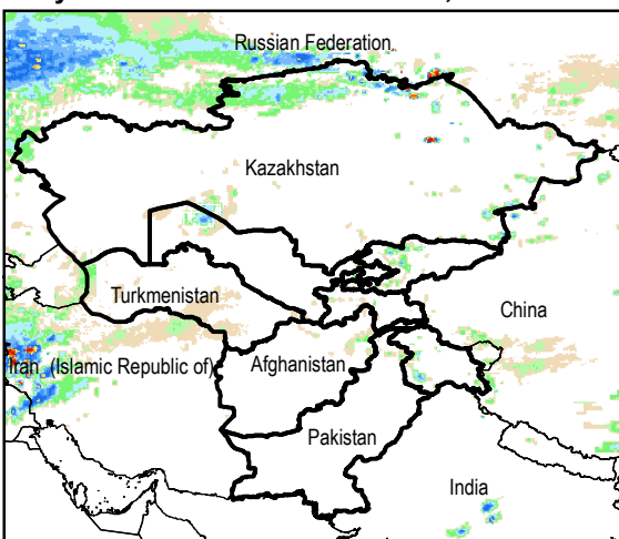
Daily Rainfall estimate for 17 Oct., 2014
