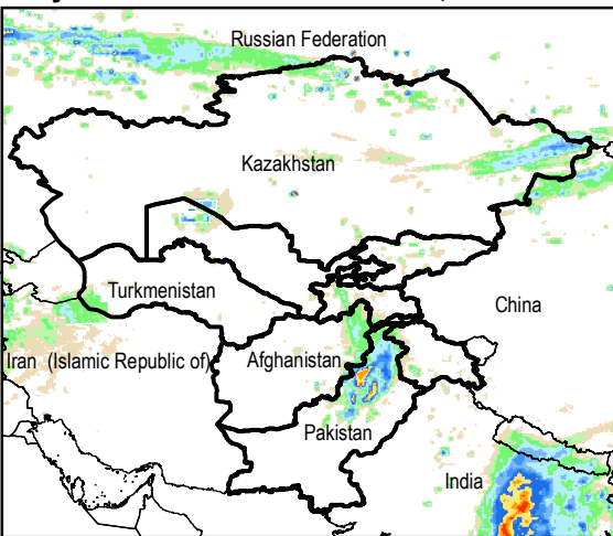
Daily Rainfall estimate for 16 Oct., 2014
