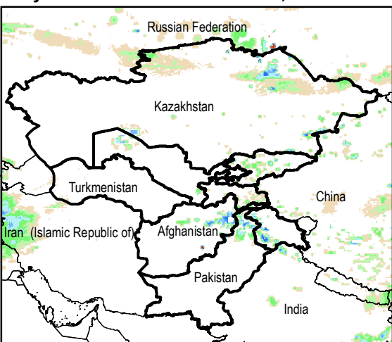
Daily Rainfall estimate for 15 Oct., 2014
