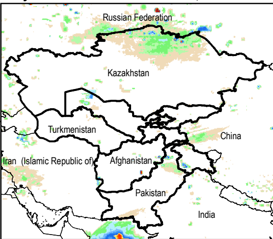
Daily Rainfall estimate for 1 Nov., 2014
