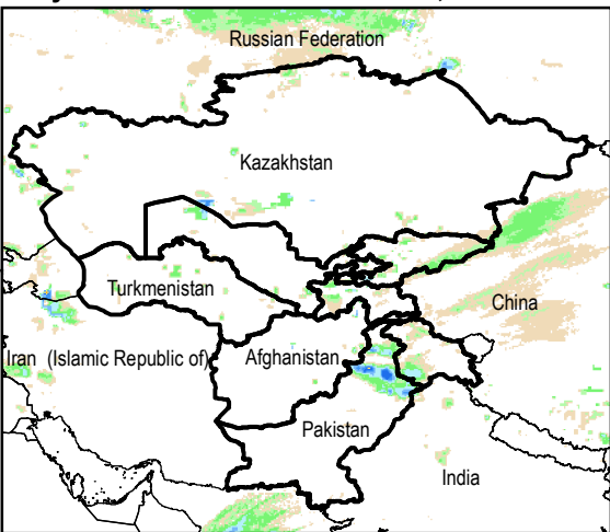
Daily Rainfall estimate for 31 Oct., 2014
