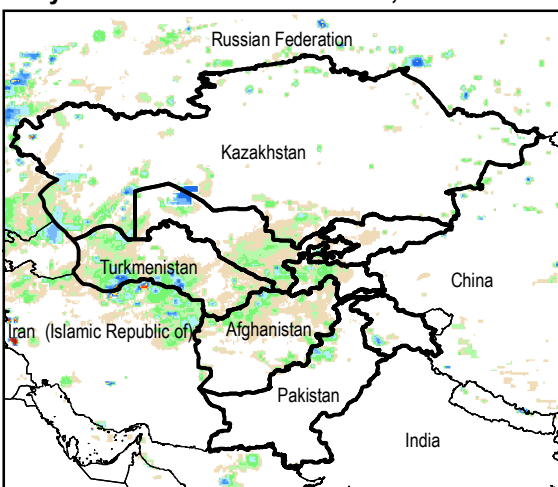
Daily Rainfall estimate for 2 Nov., 2014
