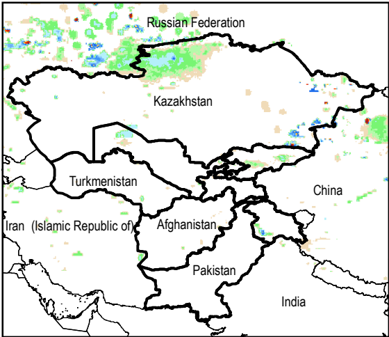
Daily Rainfall estimate for 10 Nov., 2014
