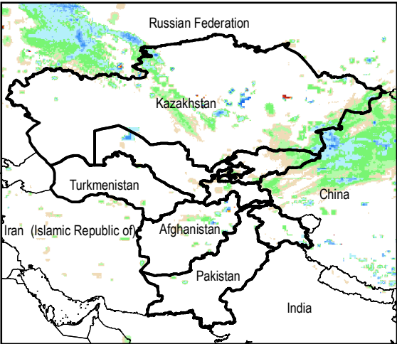
Daily Rainfall estimate for 9 Nov., 2014
