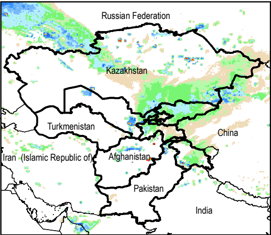
Daily Rainfall estimate for 8 Nov., 2014
