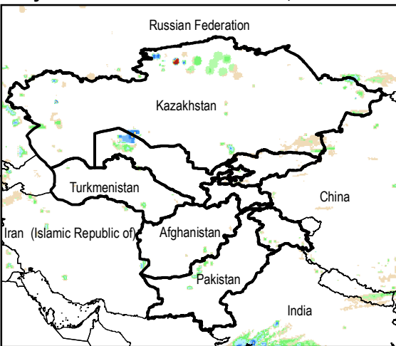
Daily Rainfall estimate for 19 Nov., 2014
