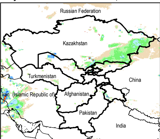
Daily Rainfall estimate for 18 Nov., 2014
