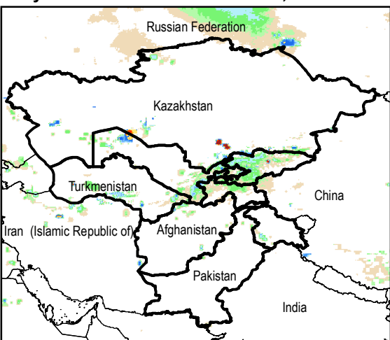
Daily Rainfall estimate for 20 Nov., 2014
