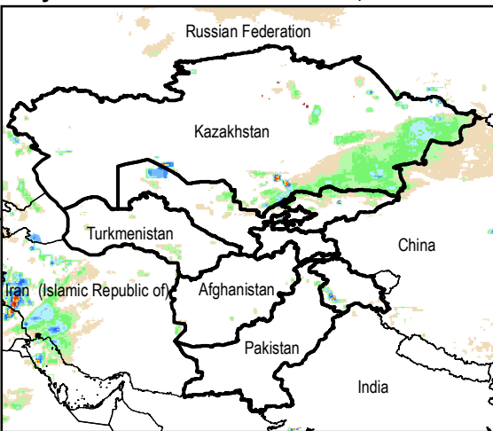
Daily Rainfall estimate for 21 Nov., 2014
