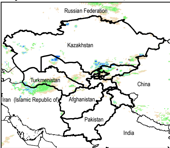
Daily Rainfall estimate for 22 Nov., 2014
