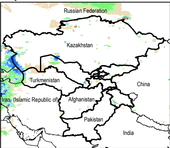
Daily Rainfall estimate for 25 Nov., 2014
