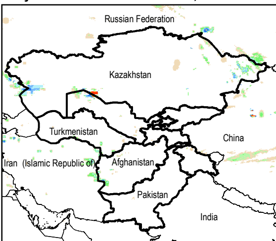
Daily Rainfall estimate for 9 Dec., 2014
