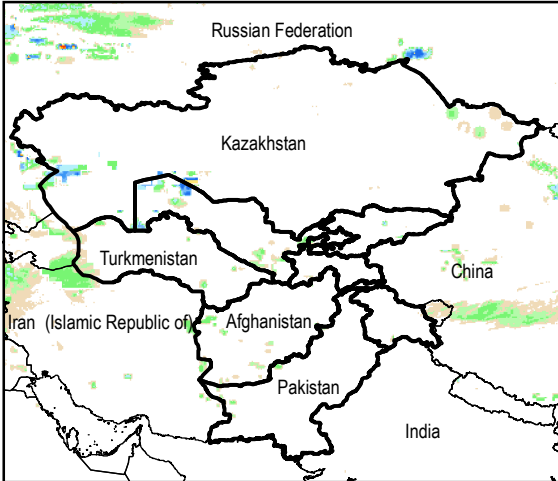
Daily Rainfall estimate for 13 Dec., 2014
