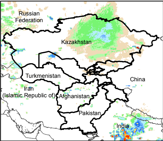
Daily Rainfall estimate for 1 Jan., 2015
