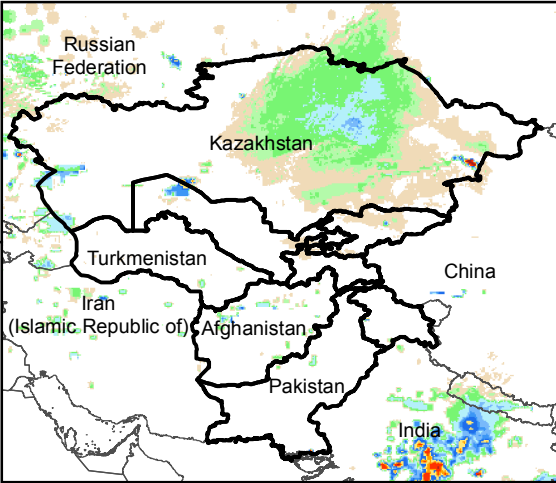
Daily Rainfall estimate for 4 Jan., 2015
