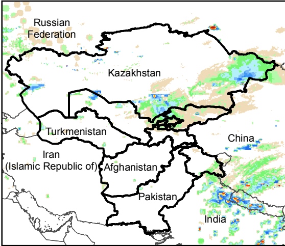
Daily Rainfall estimate for 5 Jan., 2015
