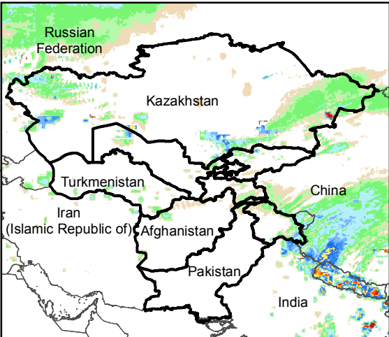
Daily Rainfall estimate for 3 Jan., 2015
