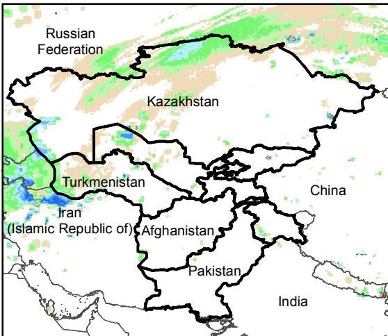
Daily Rainfall estimate for 8 Jan., 2015
