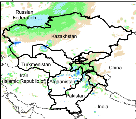
Daily Rainfall estimate for 16 Jan., 2015
