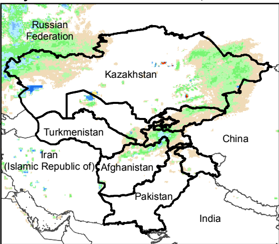
Daily Rainfall estimate for 15 Jan., 2015
