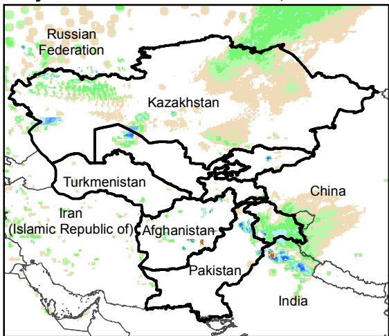
Daily Rainfall estimate for 17 Jan., 2015
