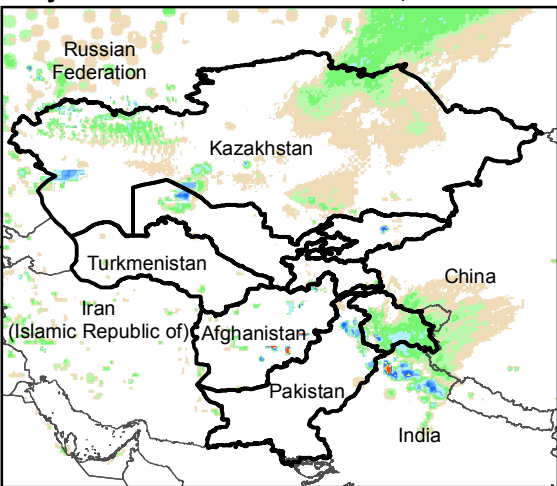
Daily Rainfall estimate for 17 Jan., 2015
