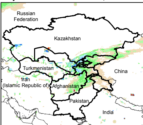
Daily Rainfall estimate for 24 Jan., 2015
