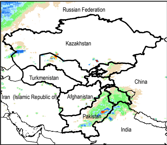
Daily Rainfall estimate for 5 Feb., 2015
