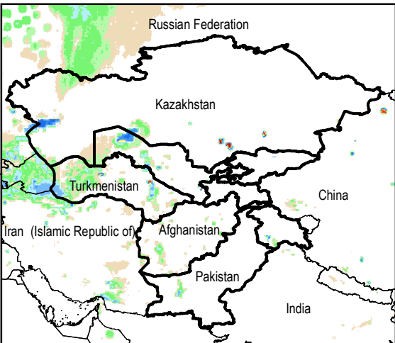
Daily Rainfall estimate for 5 Feb., 2015
