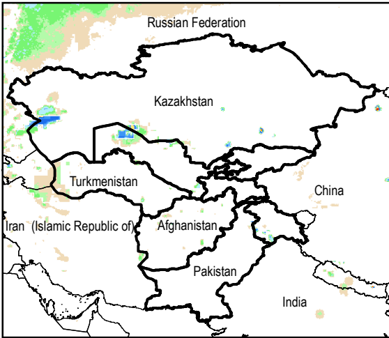
Daily Rainfall estimate for 7 Feb., 2015
